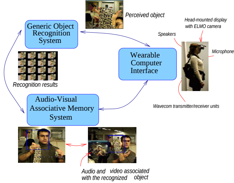
Fig. 1. System's architecture
