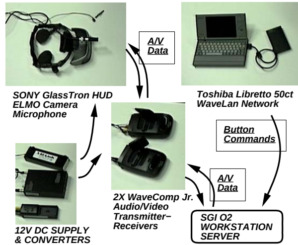
Fig. 4. The Wearable Hardware System
