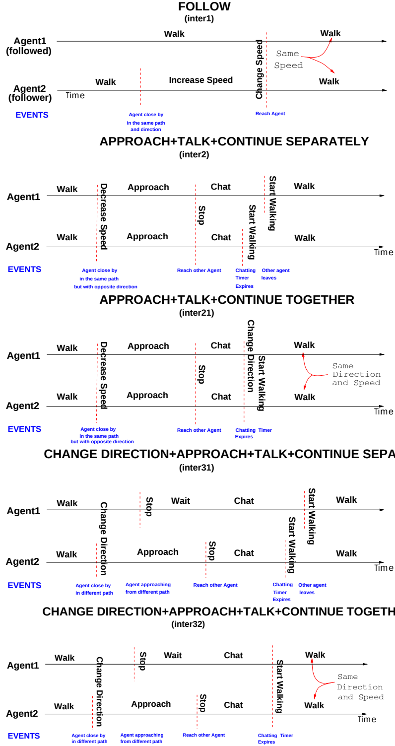
Fig. 7. Timeline of the five complex behaviors in terms of events and simple behaviors
